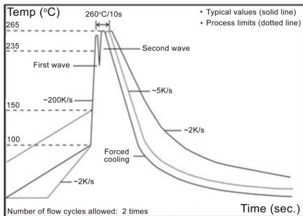
Wave Solder Temperature Condition
